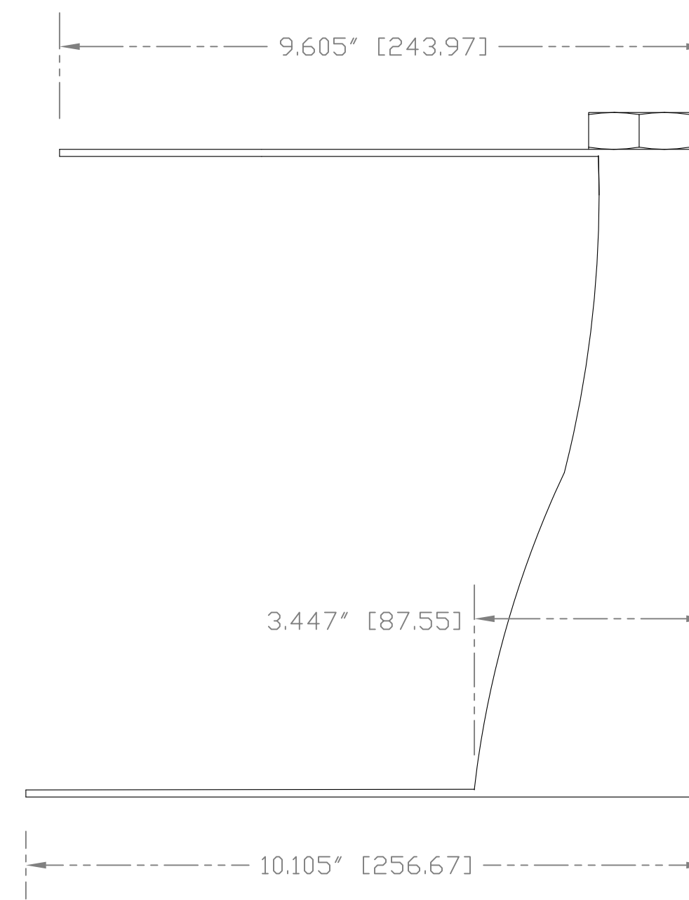
SIDE VIEW 2
