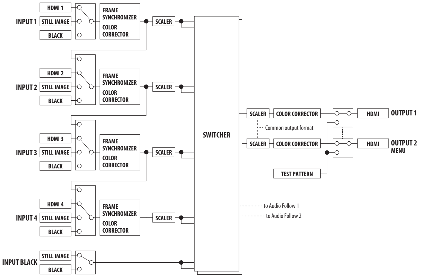
XS-42H Video Block Diagram
