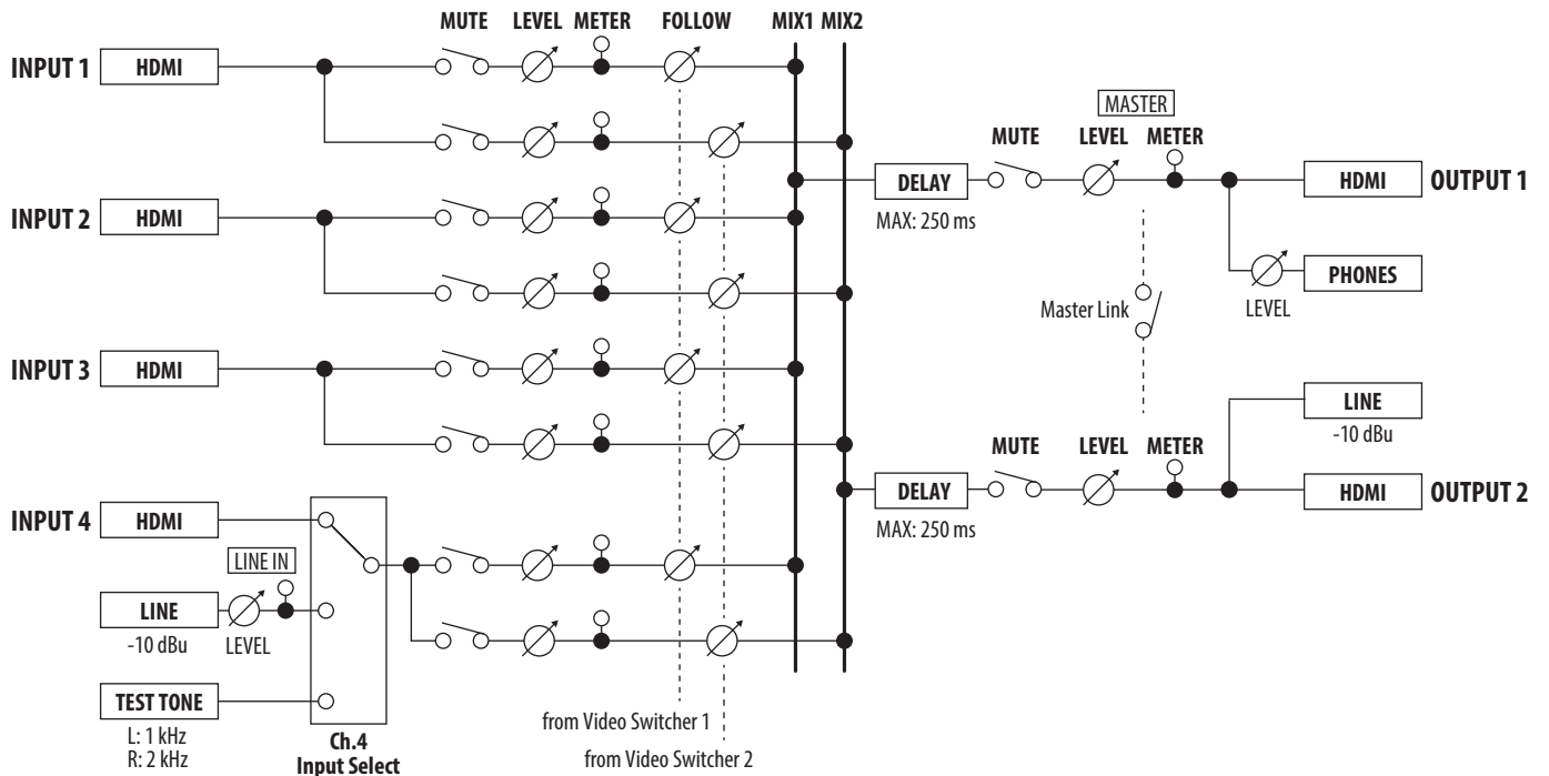
XS-42H Audio Block Diagram
