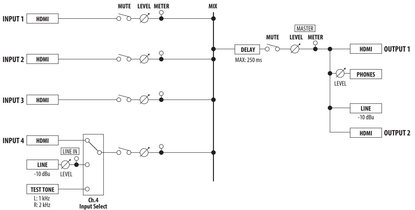
VP-42H Audio Block Diagram
