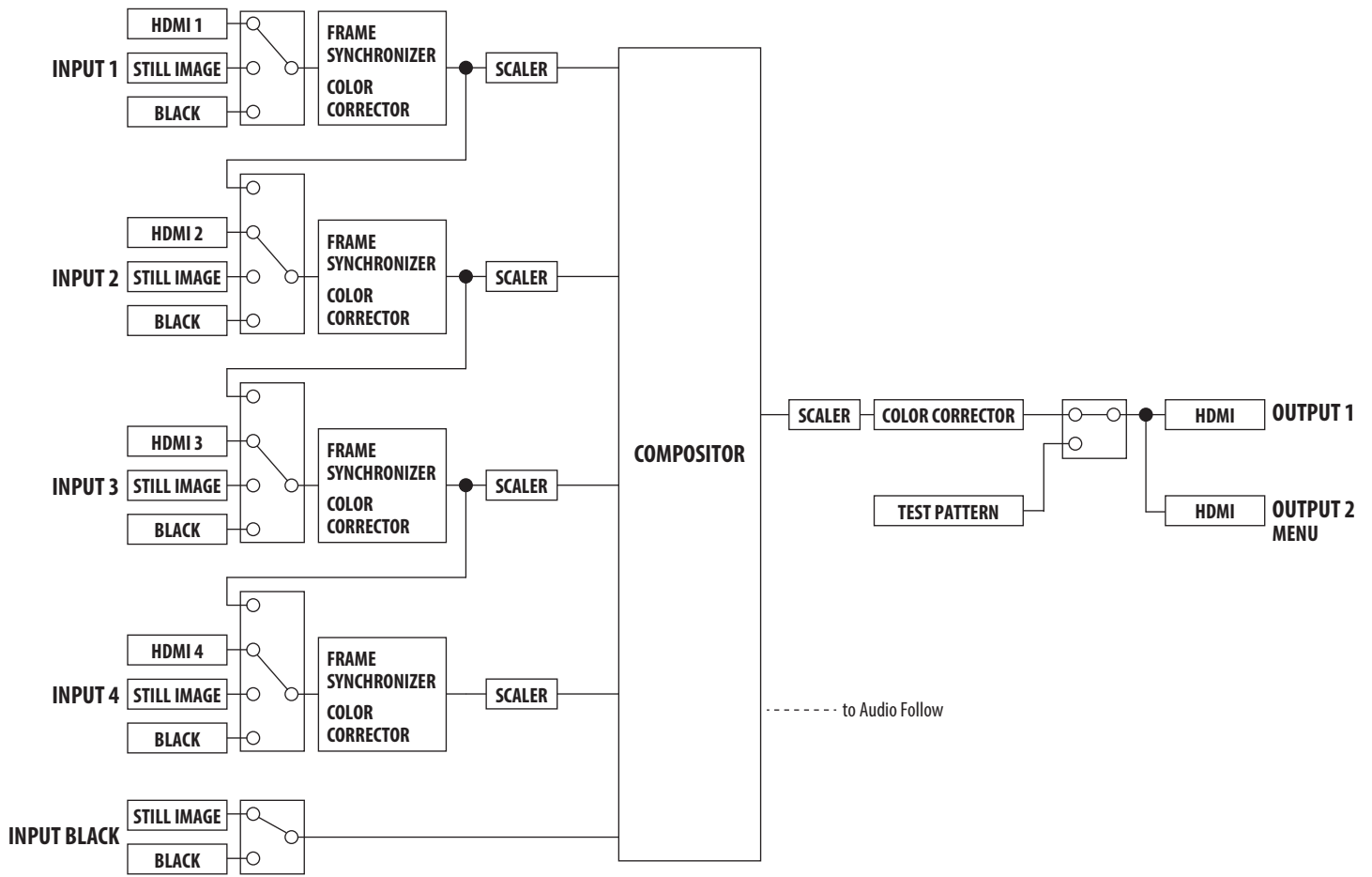
VP-42H Video Block Diagram
