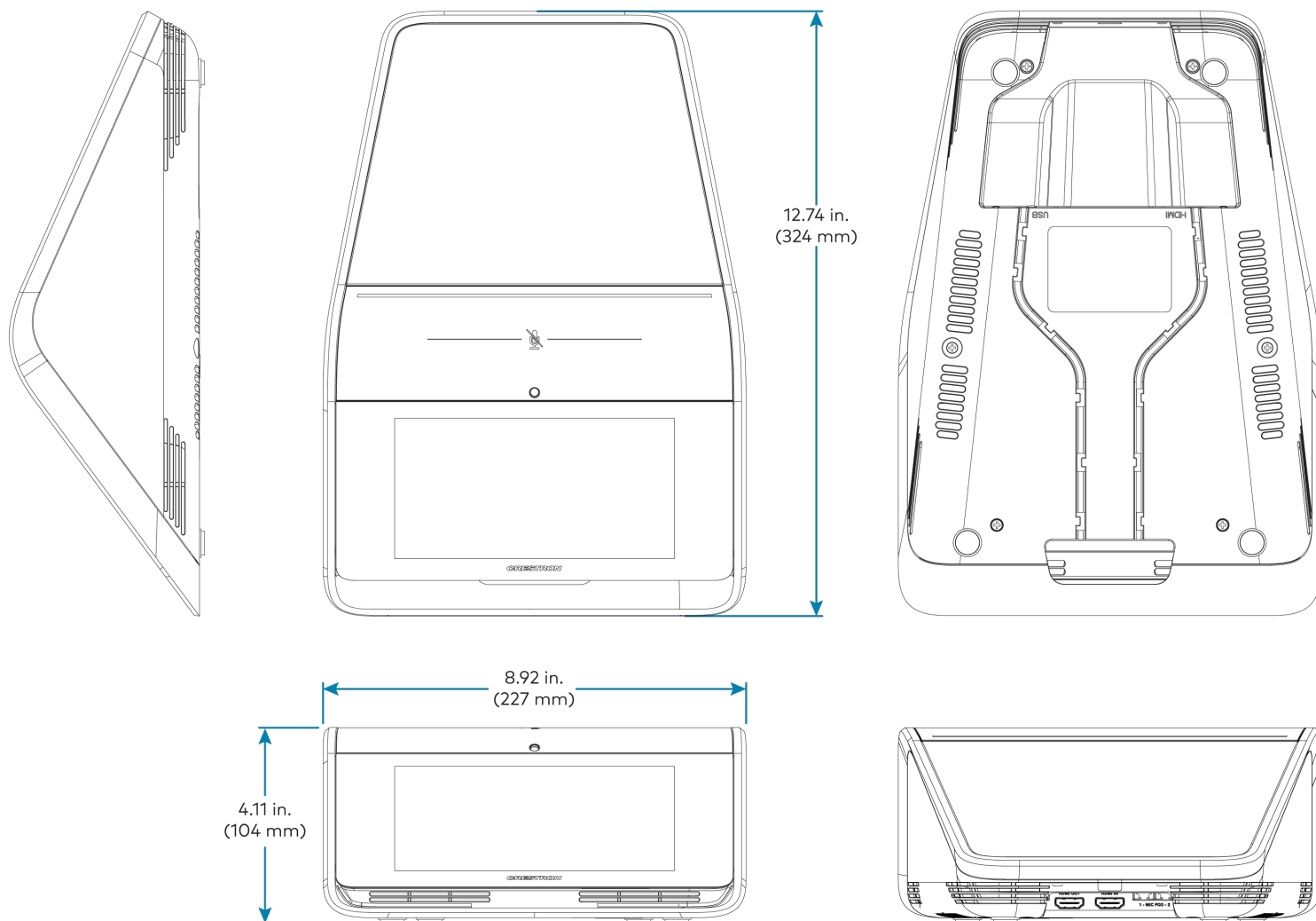
Crestron Flex Tabletop Conference Device (CCS-UC-1-T-V)
