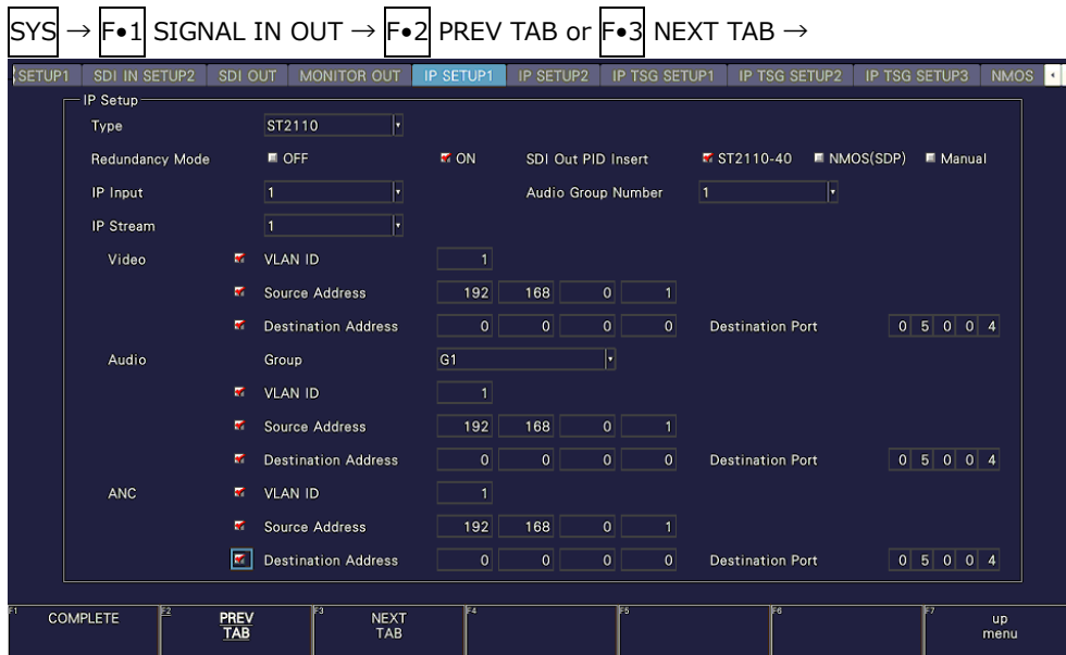
Figure 7-12 IP SETUP1 tab
