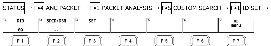
Figure 16-56 ID SET menu
