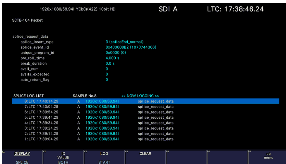
Figure 16-53 SCTE-104 detection screen (SPLICE display)
