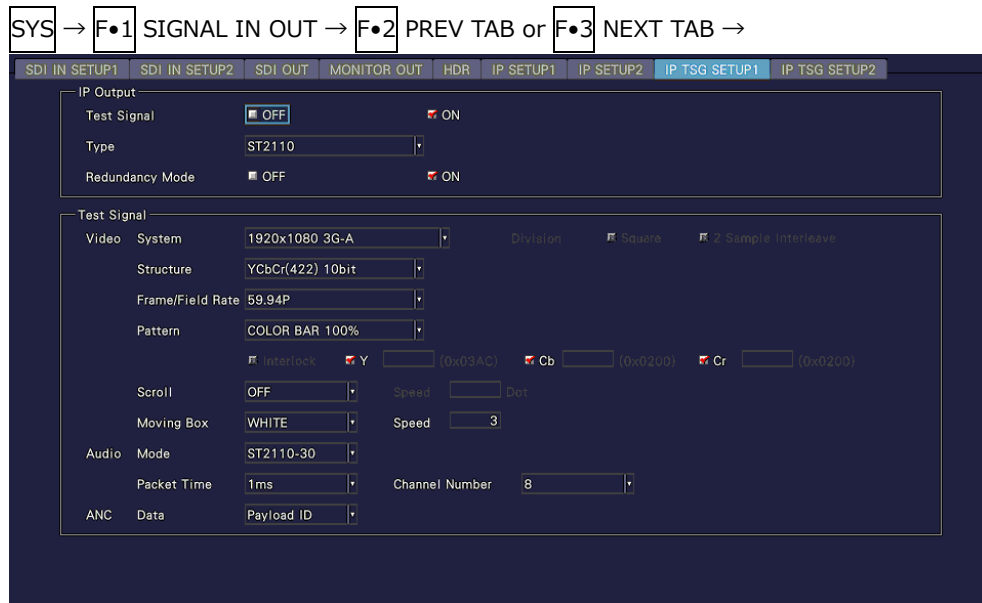
Figure 7-17 IP TSG SETUP1 tab
