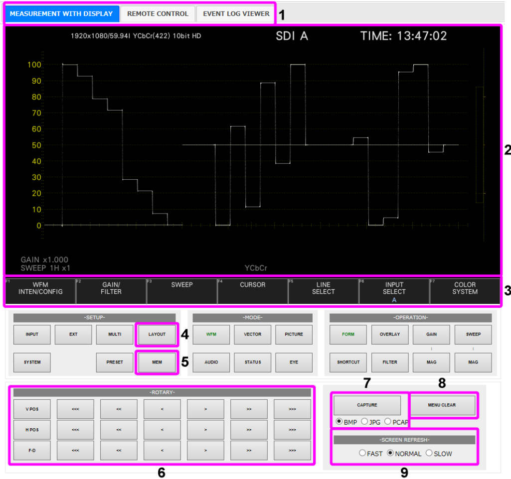
Figure 20-7 MEASUREMENT WITH DISPLAY
