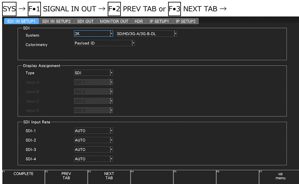
Figure 7-5 SDI IN SETUP1 tab
