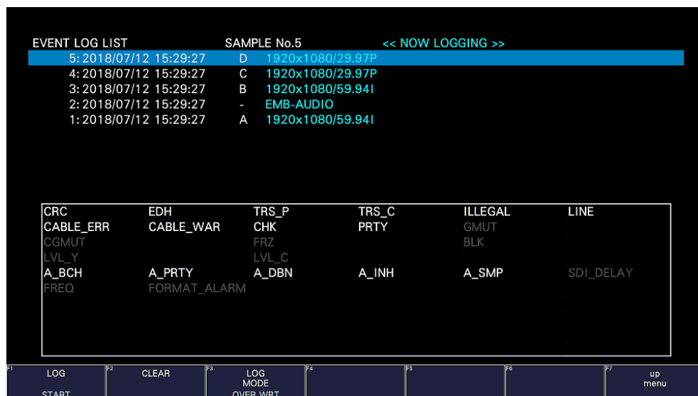
Figure 15-24 Event log display
