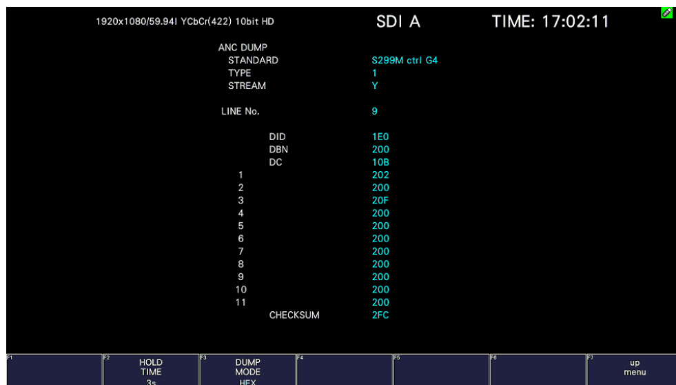
Figure 16-32 Ancillary dump screen
