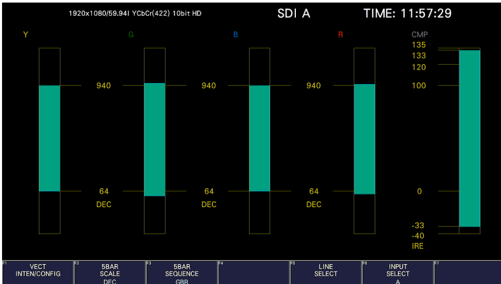
Figure 11-25 Selecting the scale unit
