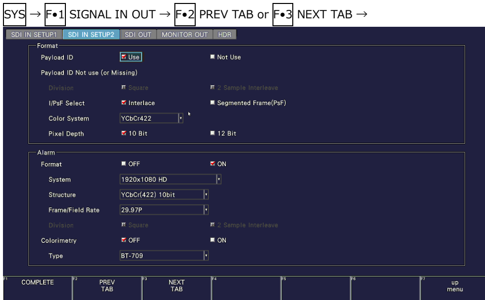
Figure 7-6 SDI IN SETUP2 tab
