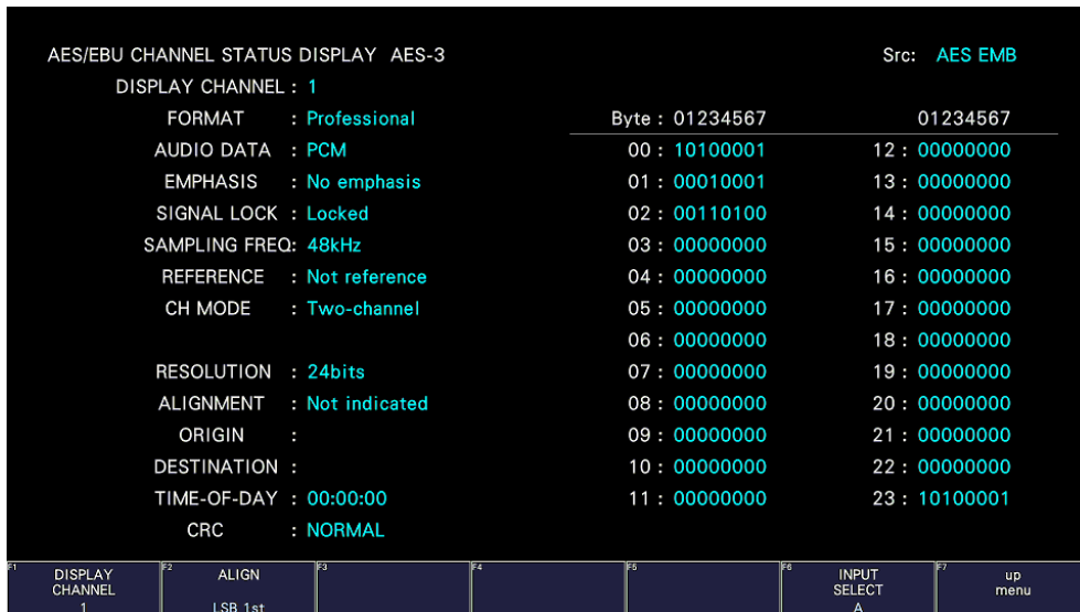
Figure 15-32 Channel status display
