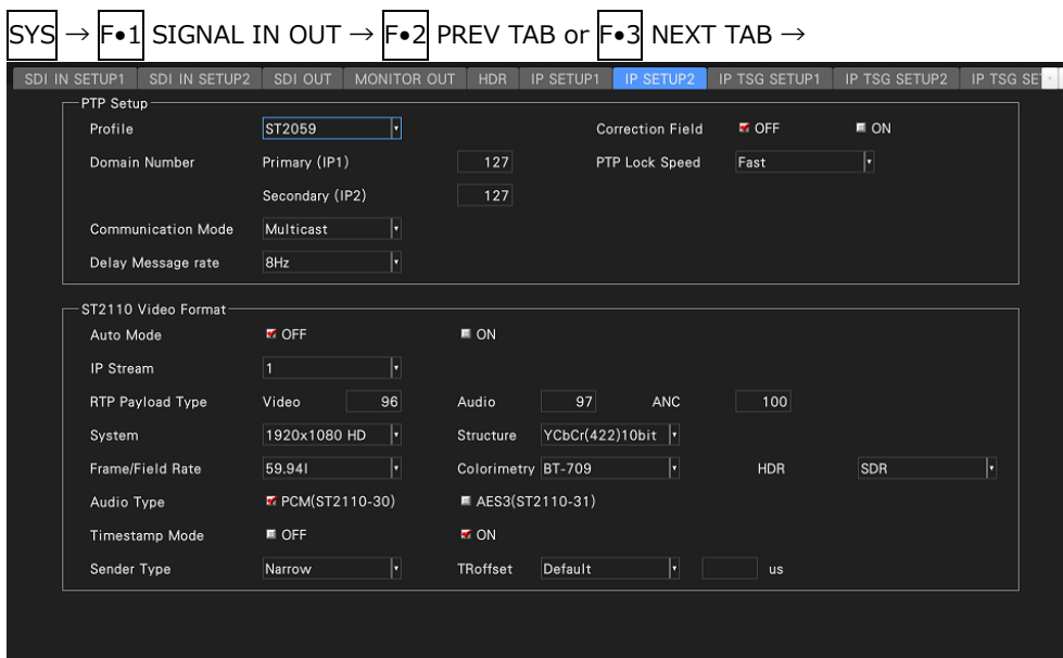
Figure 7-15 IP SETUP2 tab
