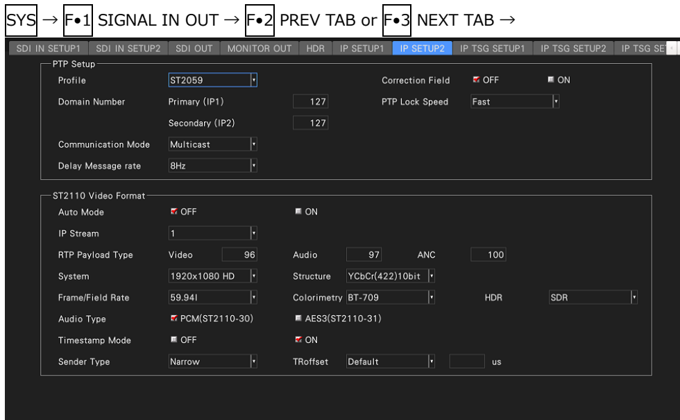
Figure 7-14 IP SETUP2 tab
