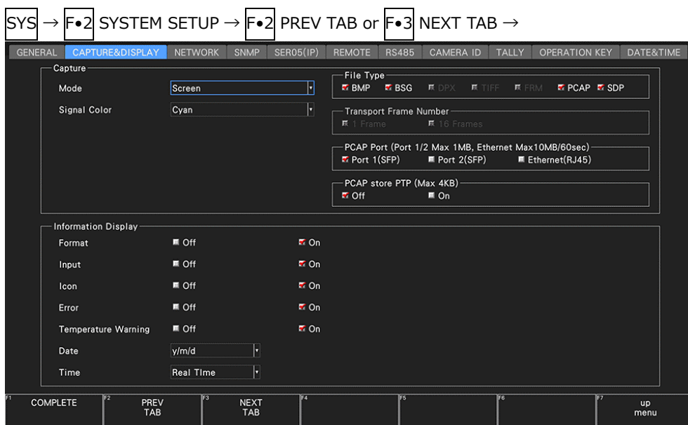
Figure 7-26 CAPTURE & DISPLAY tab
