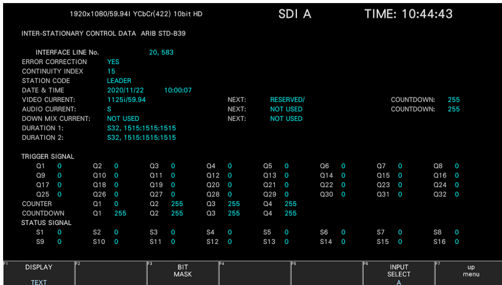
Figure 16-40 Inter-stationary control signal screen (TEXT)
