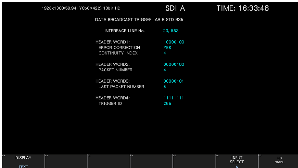
Figure 16-43 Data broadcast trigger signal screen
