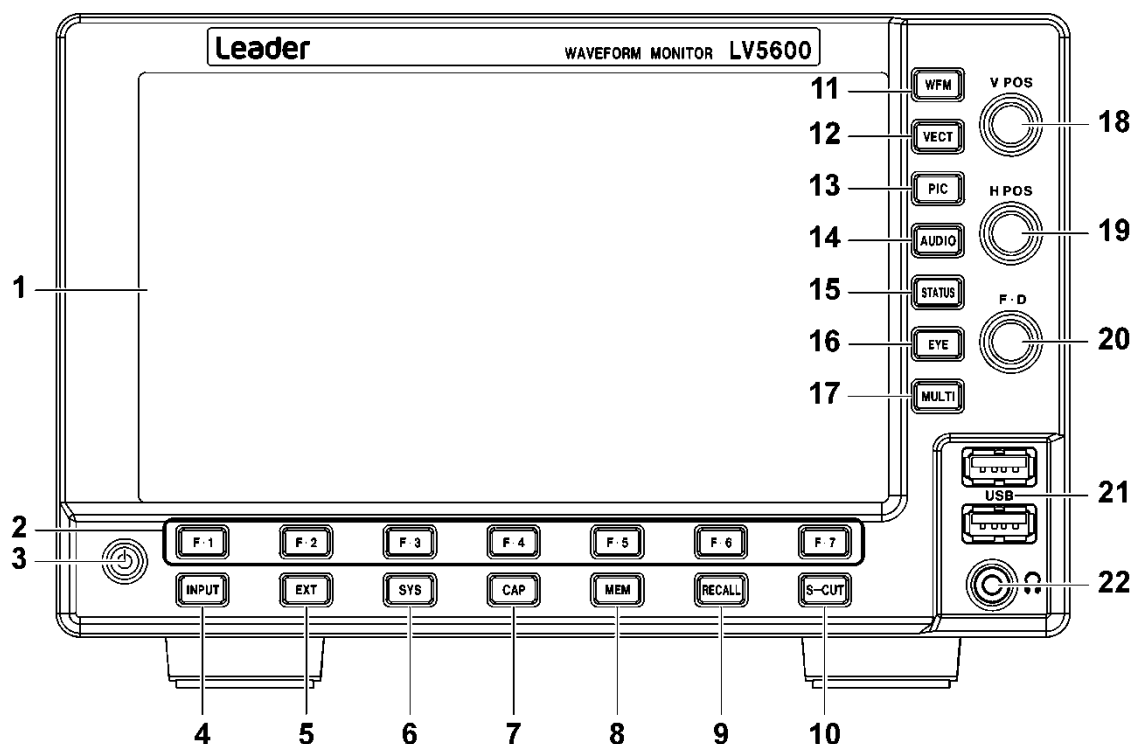
Figure 4-1 LV5600 front panel
