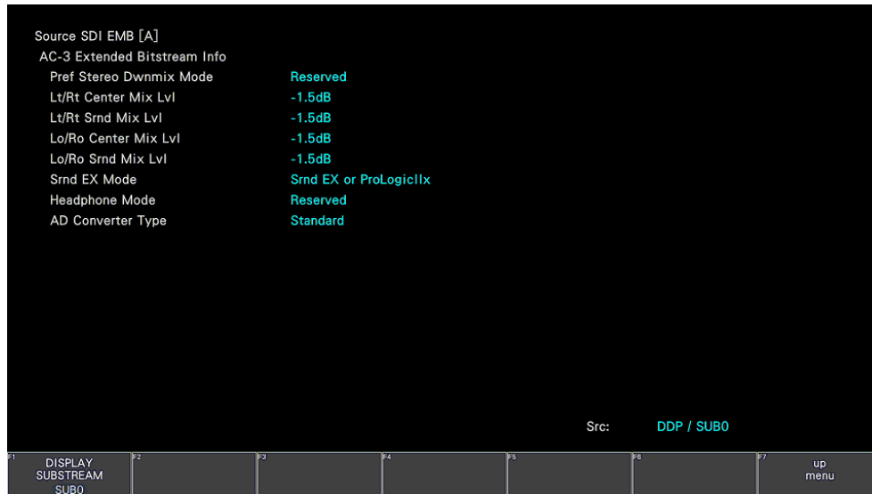
Figure 15-31 Dolby Digital Plus EBI metadata display
