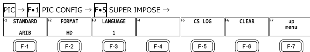
Figure 13-18 SUPER IMPOSE menu
