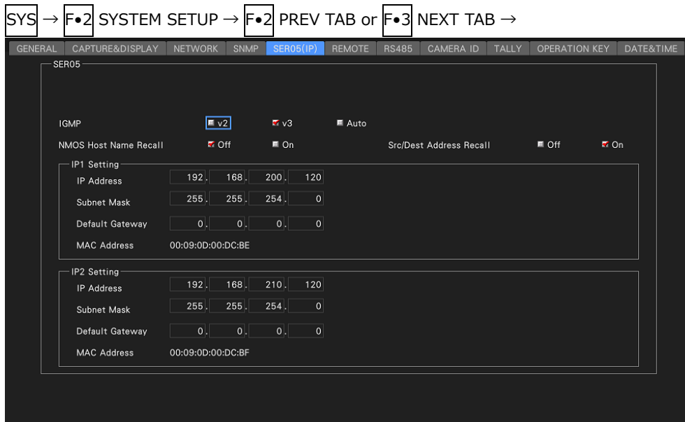
Figure 7-33 SER05 (IP) tab
