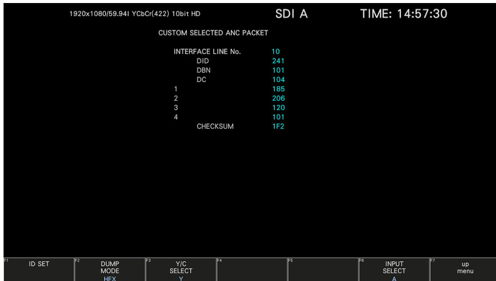
Figure 16-55 Custom search screen
