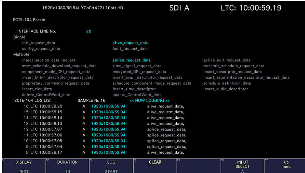
Figure 16-51 SCTE-104 detection screen (TEXT display)
