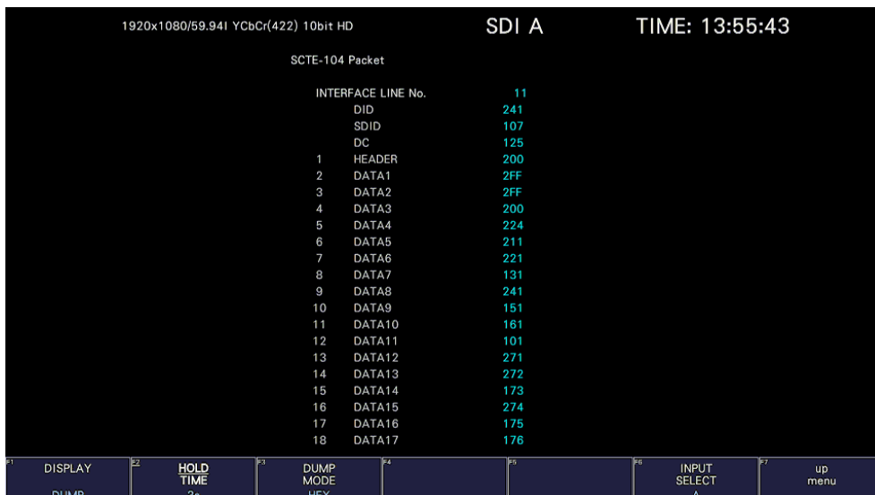
Figure 16-52 SCTE-104 detection screen (DUMP display)
